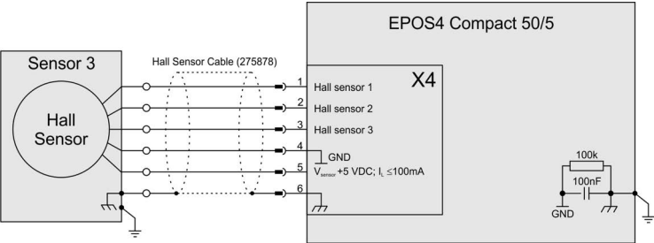
Figure 5-65Hall sensors (Sensor 3)
