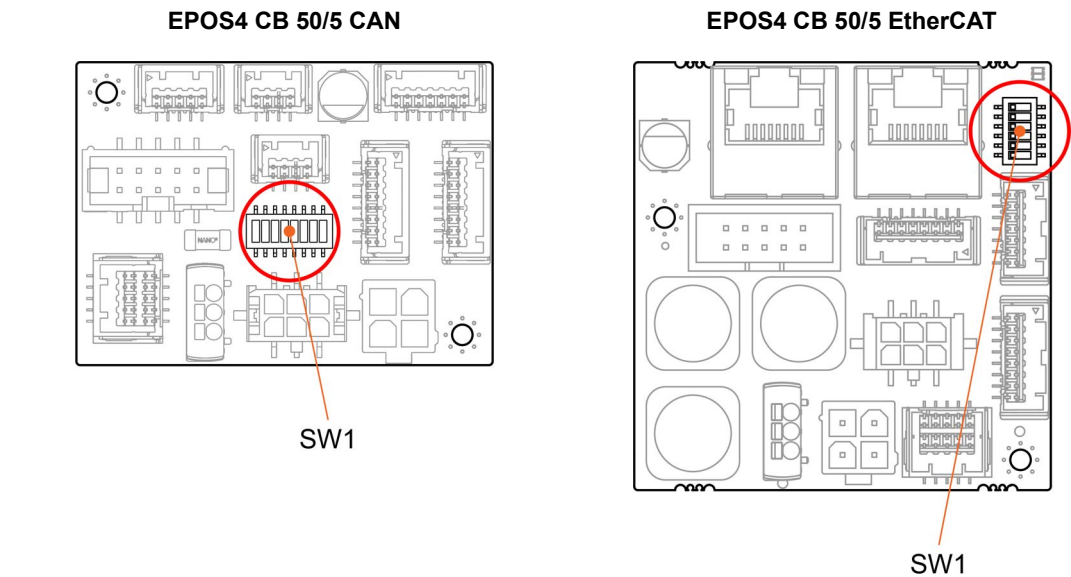
Figure 3-26 DIP switch SW1
