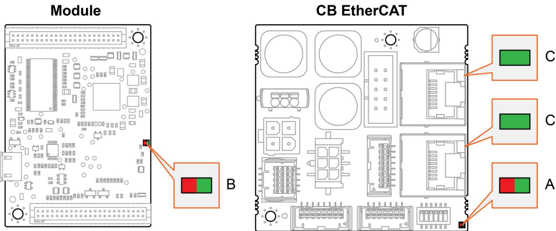
Figure 3-53 LEDs – Location
