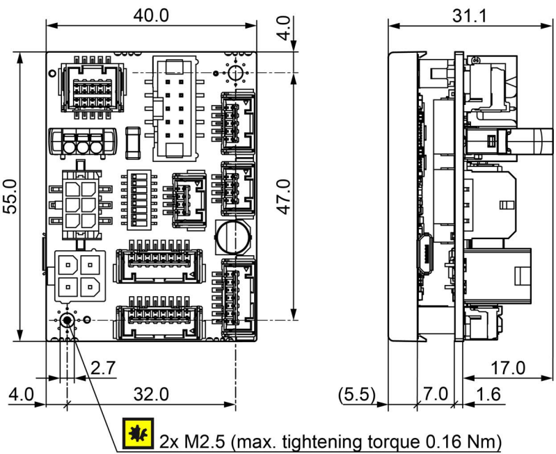
Figure 2-8 EPOS4 Compact 50/5 CAN – Dimensional drawing [mm]
