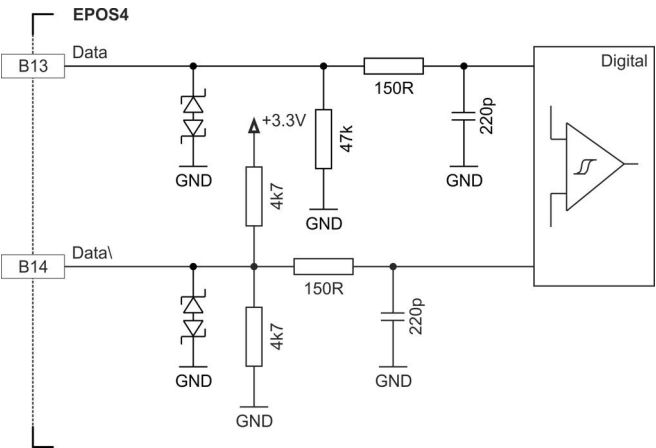
Figure 3-36 SSI absolute encoder data input
