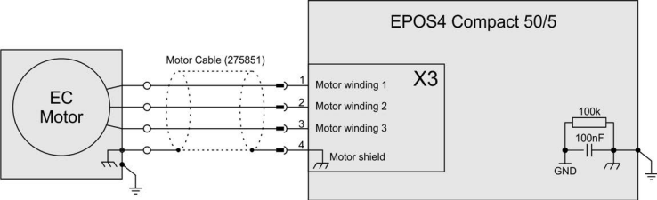
Figure 5-64EC (BLDC) motor
