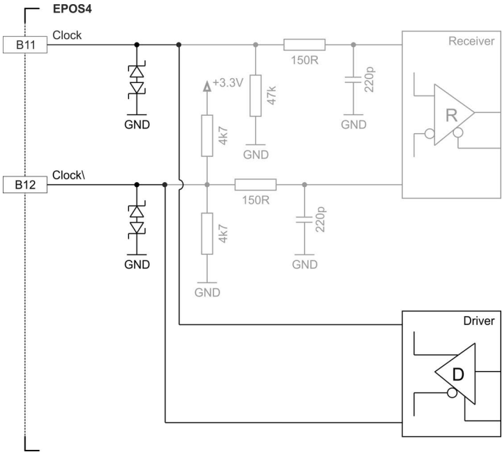
Figure 3-37 SSI absolute encoder clock output
