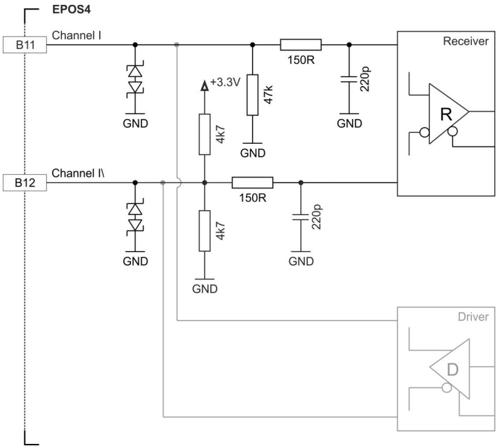
Figure 3-31 Digital incremental encoder input circuit Ch I
