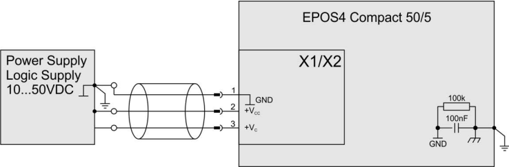
Figure 5-62Power & logic supply
