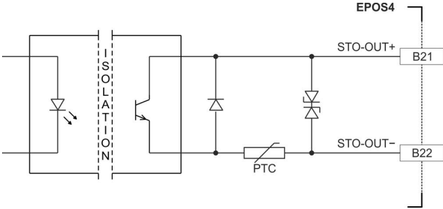
Figure 3-48 STO-OUT circuit
