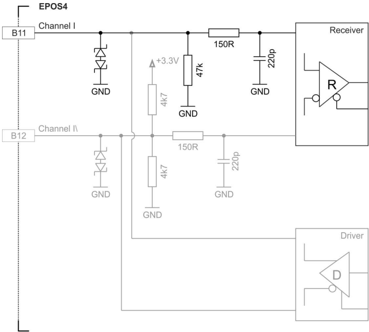
Figure 3-33 Digital incremental encoder input circuit Ch I
