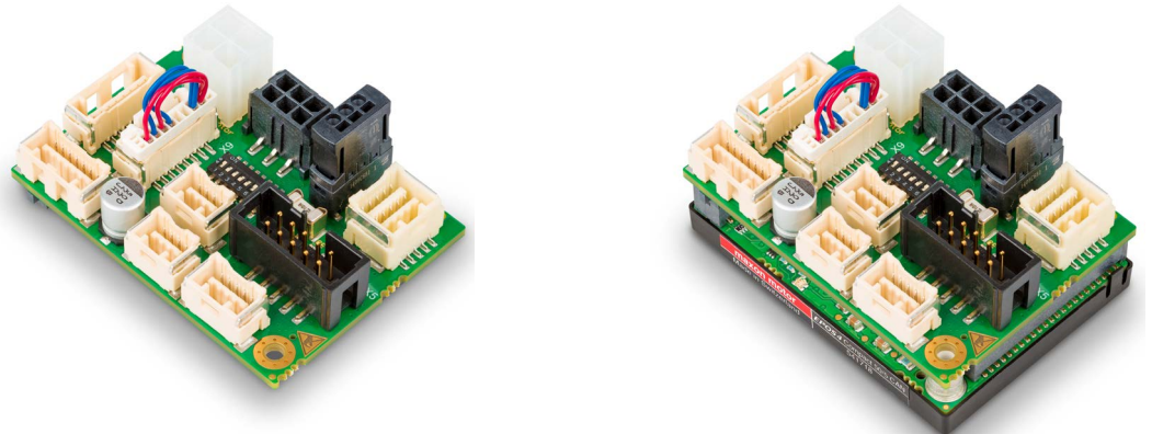
Figure 3-12 EPOS4 CB 50/5 CAN (left) / EPOS4 Compact 50/5 CAN (right)
